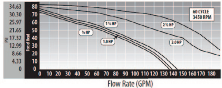
Pressure v. Flow Rate @ Max Speed
